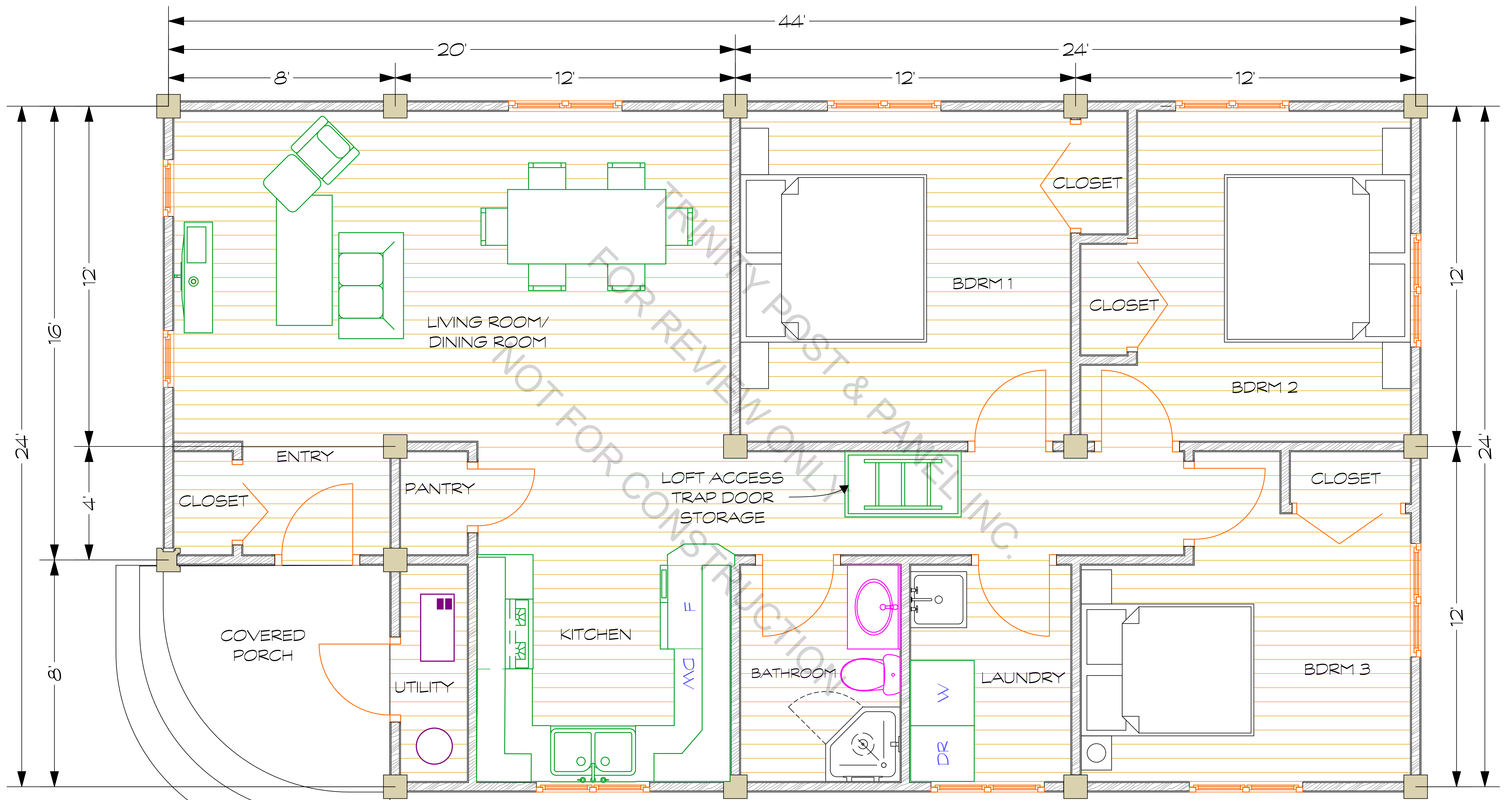
TRINITY RANCHER 3 BEDROOM + LOFT 1018 SQ FT
